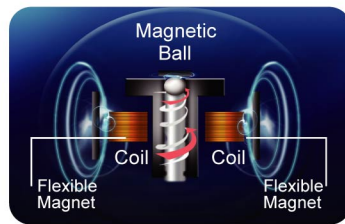
Twister Bearing (100K hours lifetime)
